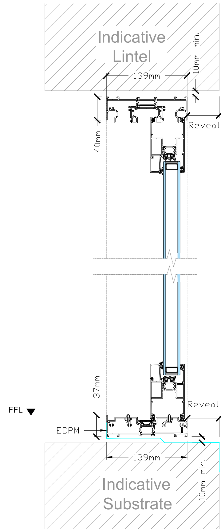
Section - AA 1:4
